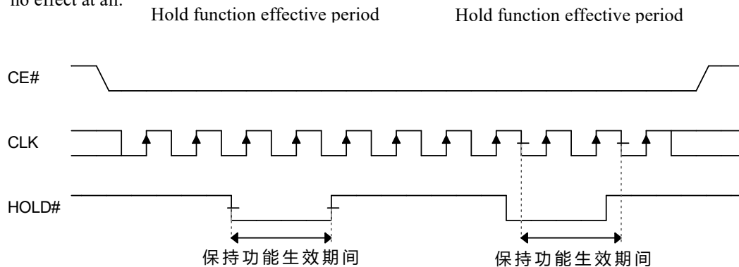
Figure 12: Hold Mode Functional Sequence Diagram
