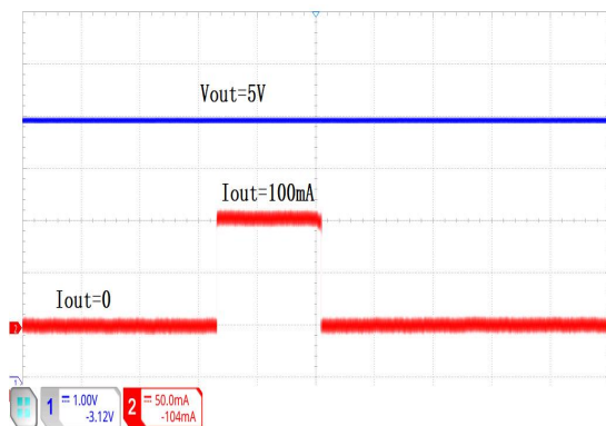
Load Transient Response (VIN=24V, VOUT=5V, IOUT=0~100mA)
