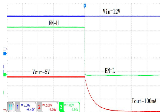
EN OFF (VIN=12V, VOUT=5V, RLOAD=50Ω, Time (10ms/div))
