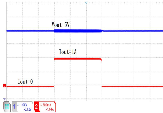
Load Transient Response (VIN=24V, VOUT=5V, IOUT=0~1A)
