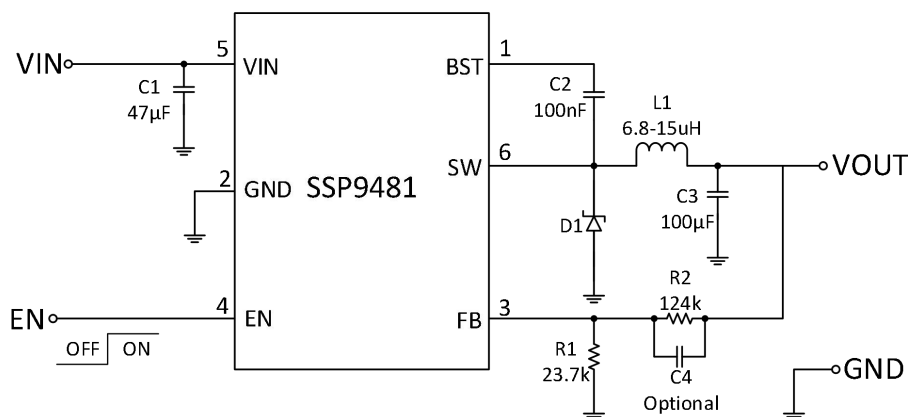
5V output typical application circuit
