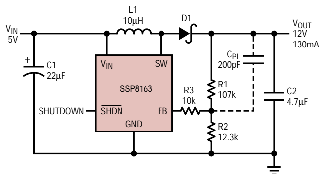
Figure 10. 5V to 12V Boost Converter with 4.7μF Ceramic Output Capacitor, C_{PL} Added to Increase Phase Margin
