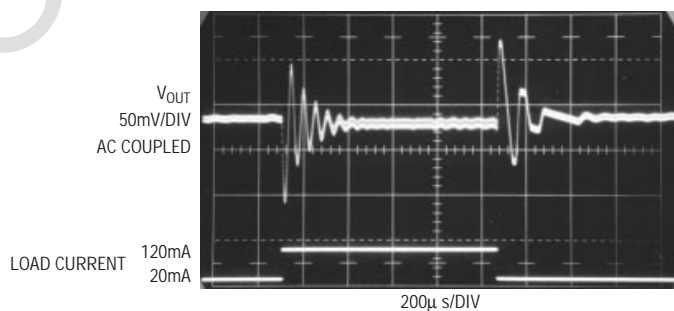
Figure 14. 5V Output SEPIC with 10μF Ceramic Output Capacitor. No C_{PL} . V_{IN} = 4V
