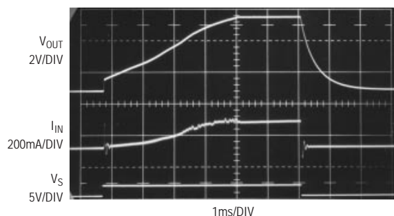
Figure 19. Increasing C_S to 33nF Further Reduces Inrush Current. R_{LOAD} = 50\Omega
