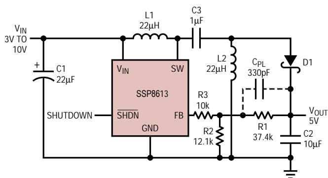
Figure 13. 5V Output SEPIC with Ceramic Output Capacitor. C_{PL} Adds Phase Margin
