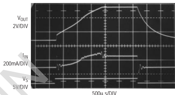
Figure 18. Soft-Start Components in Figure 17's SEPIC Reduces Inrush Current. C_{SS} = 10nF , R_{LOAD} = 50\Omega
