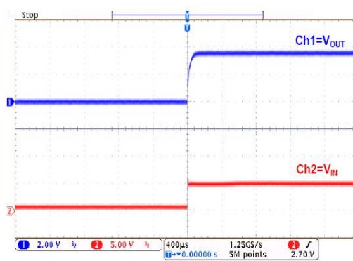
Power-Up at V_{OUT}=3.6V SSP7903P36 ( I_{OUT}=1A )
