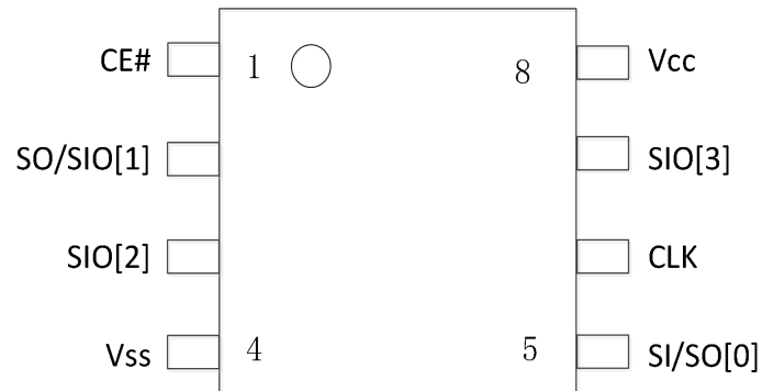
Figure 1: Package Information
