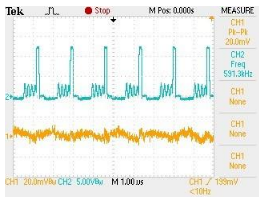
STEADY STATE OPERATION (VIN=12V,VOUT=1.2V,IOUT=100mA)
