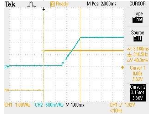
START UP (VIN=12V,VOUT=1.2V)
