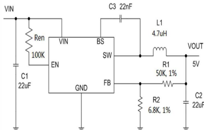
Basic Application Circuit For VOUT=5V
