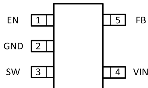
SOT23-5(Top View)
